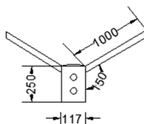
2. Pole cap with double arms
