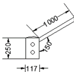
1. Pole cap with single arm
